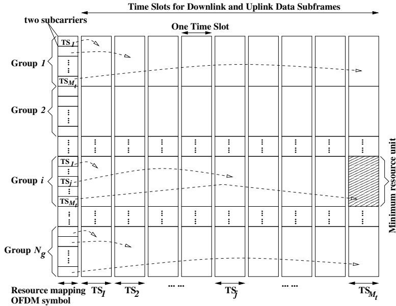
Fig. 2. A new resource mapping scheme.
