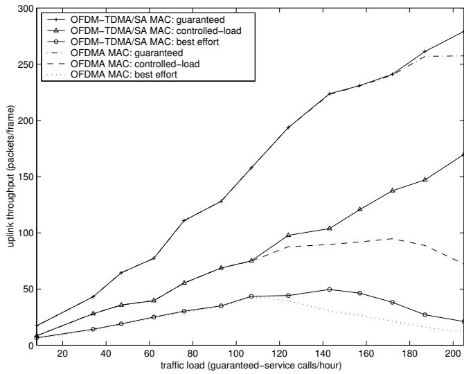
Fig. 7. The uplink throughput of different services.
