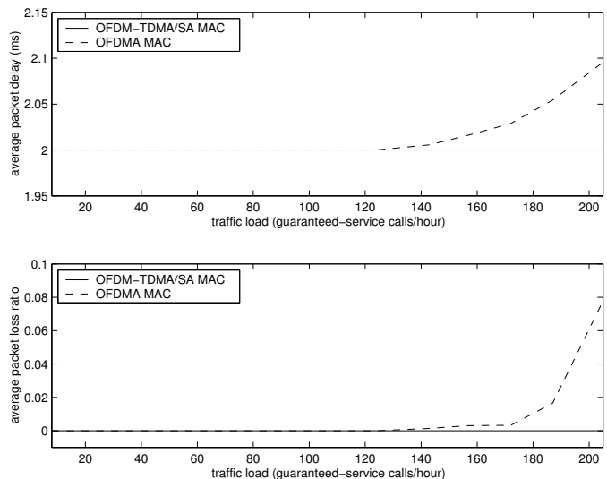
Fig. 4. The average packet delay and packet loss ratio of guaranteed service.
