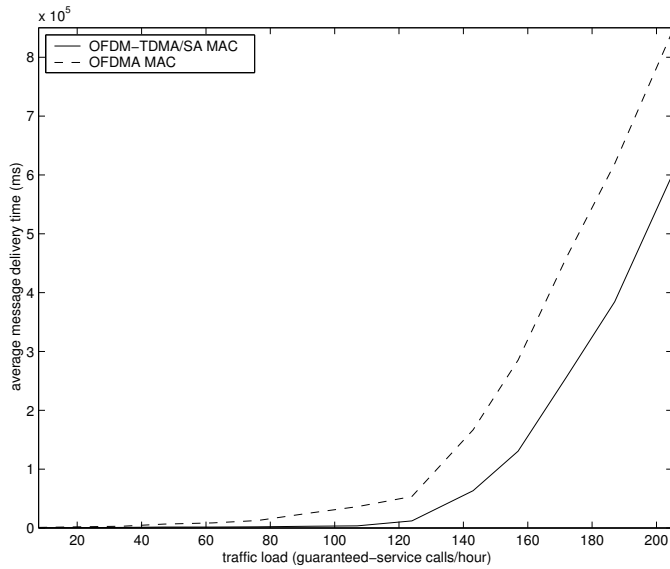
Fig. 6. The average message delivery time of best effort service.
