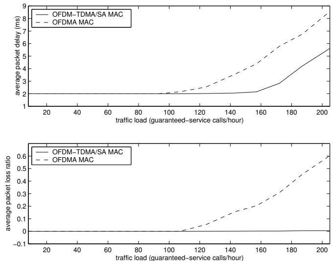
Fig. 5. The average packet delay and packet loss ratio of controlled-load services.
