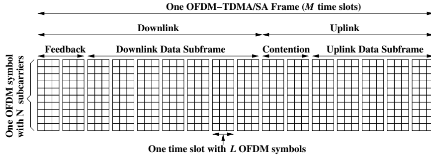
Fig. 1. OFDM-TDMA/SA frame structure.
