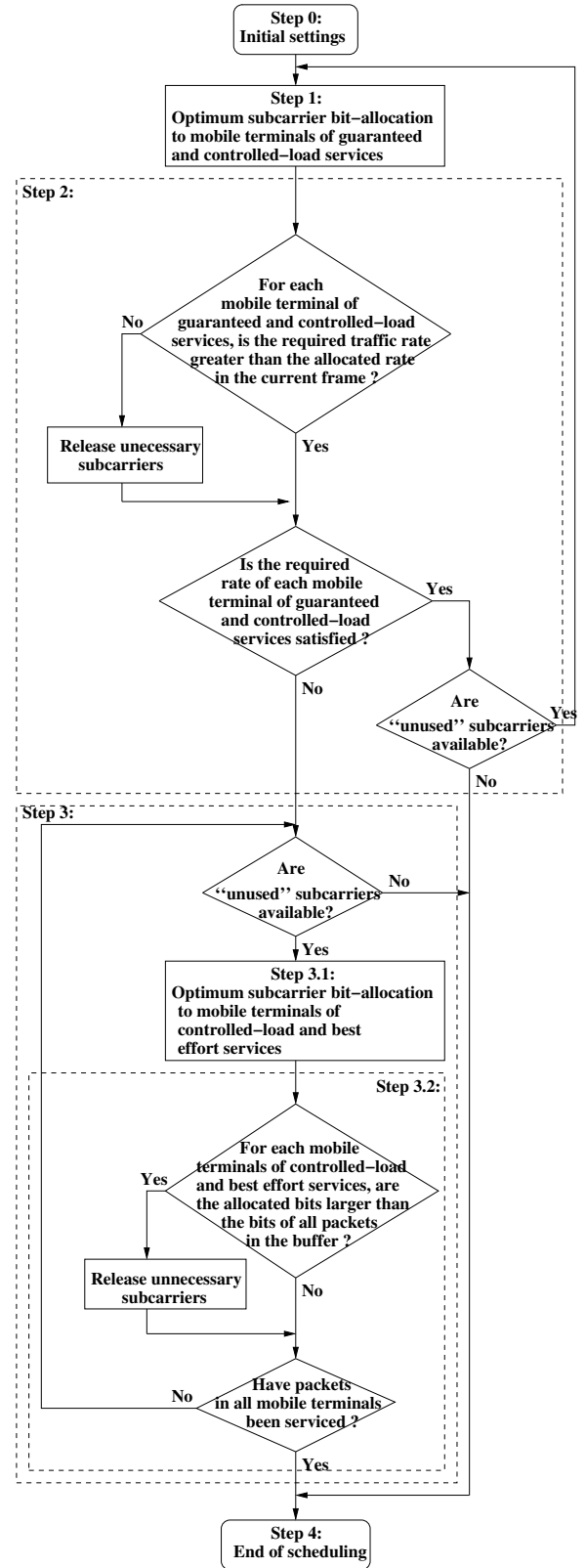
Fig. 3. The hierarchical scheduling scheme.
